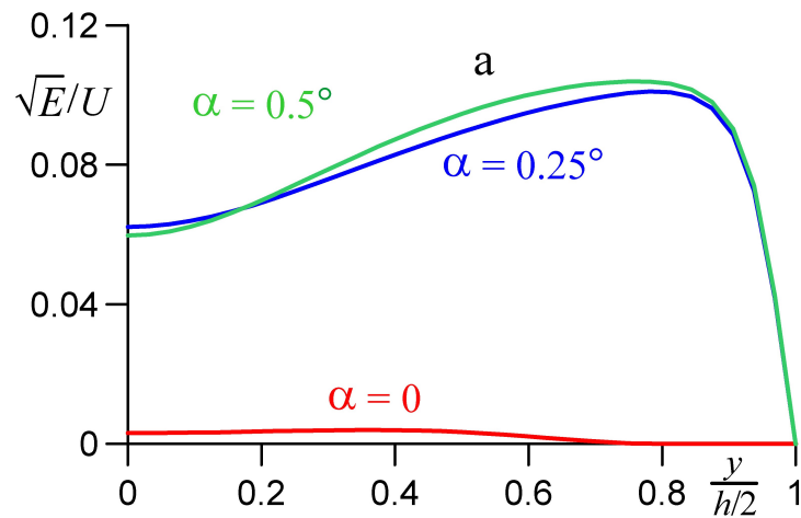
Channel height distribution of turbulence intensity at the end of the heat exchange part of the cold coolant channel
